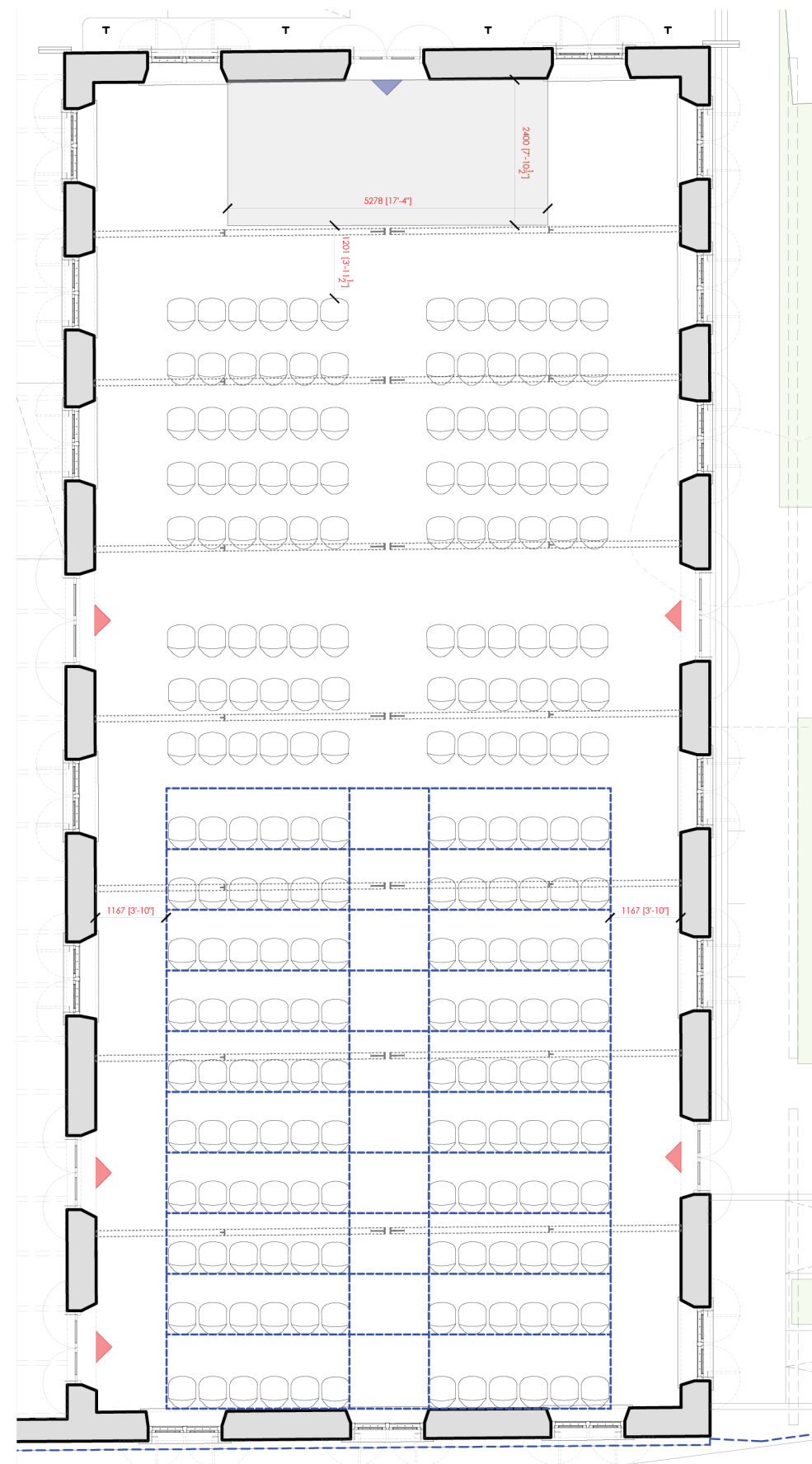
Proscenium Layout-2 Capacity- 216 Seats
