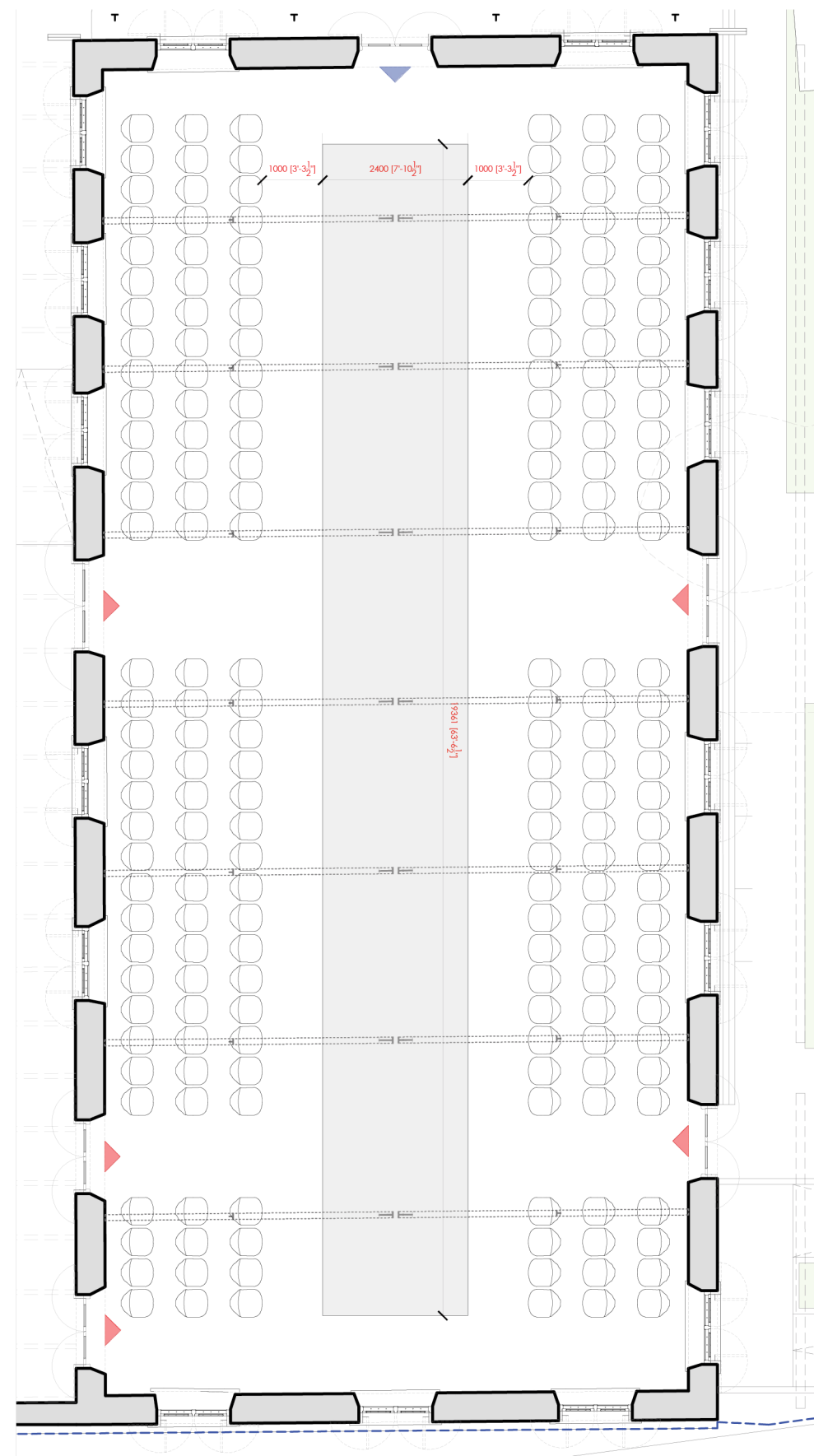
Traverse Stage Layout Capacity- 198 Seats on ground
