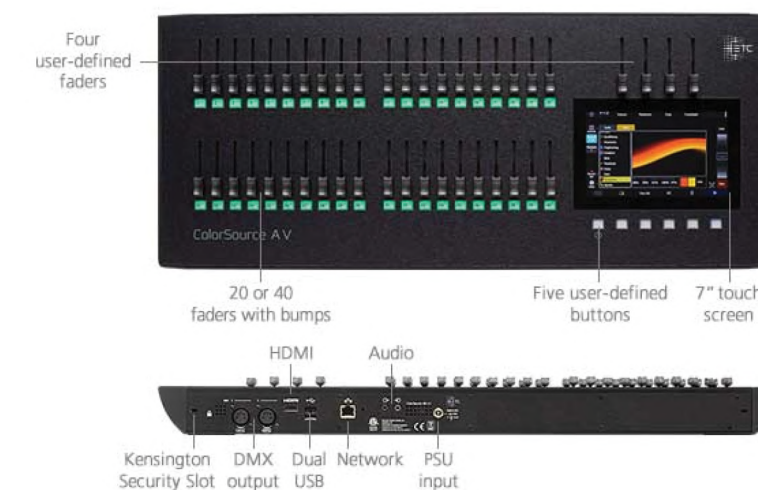
Colour Source AV- Lighting Console ETC
