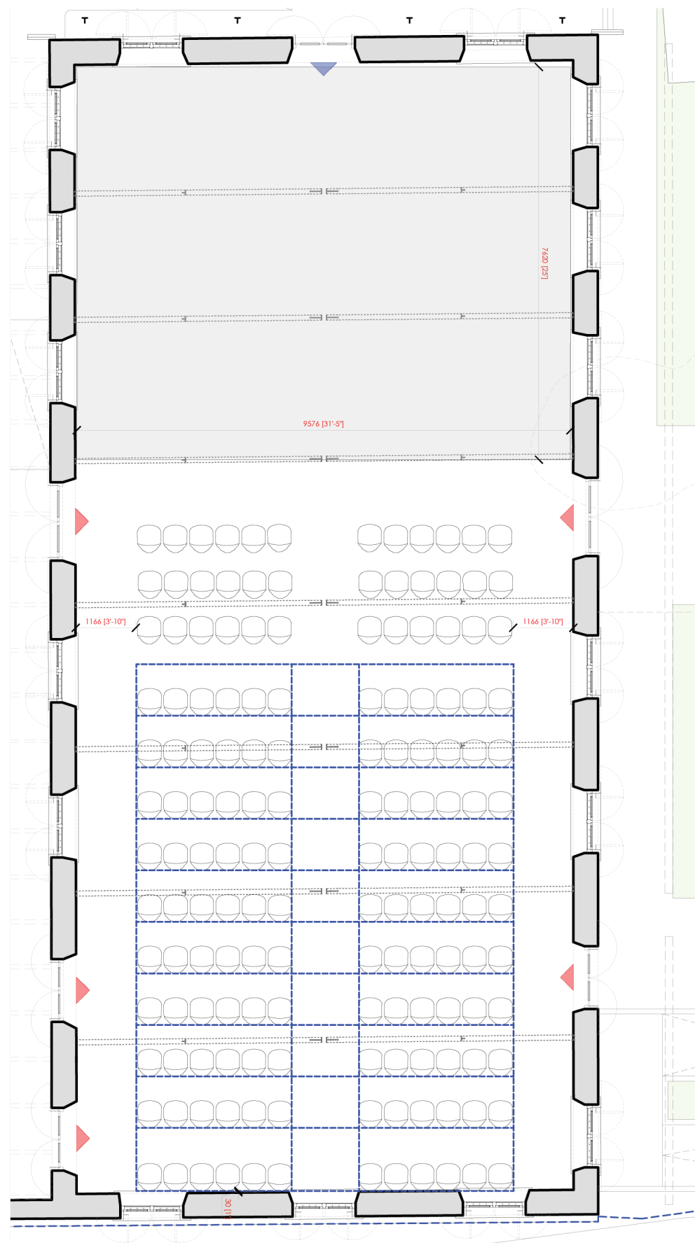
Proscenium Layout-1 Capacity- 156 Seats
